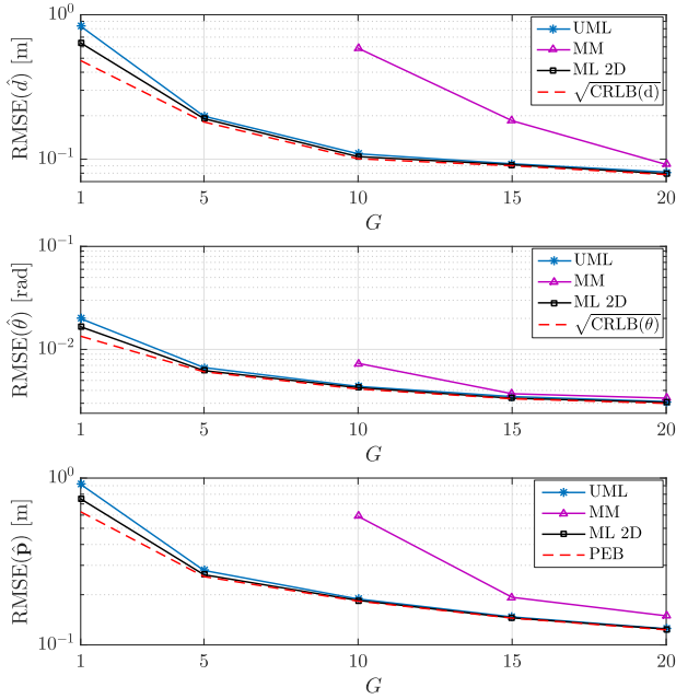
Fig. 4. RMSEs of the estimated d , \theta , and \mathbf{p} versus CRLBs as function of the transmissions G for SNR = 5 dB in LOS condition.
