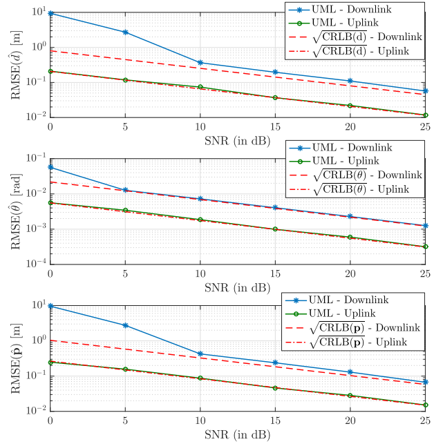
Fig. 5. RMSEs of the estimated d , \theta , and \mathbf{p} versus CRLBs as function of the SNR for G = 1 in LOS condition for both uplink and downlink channels.
