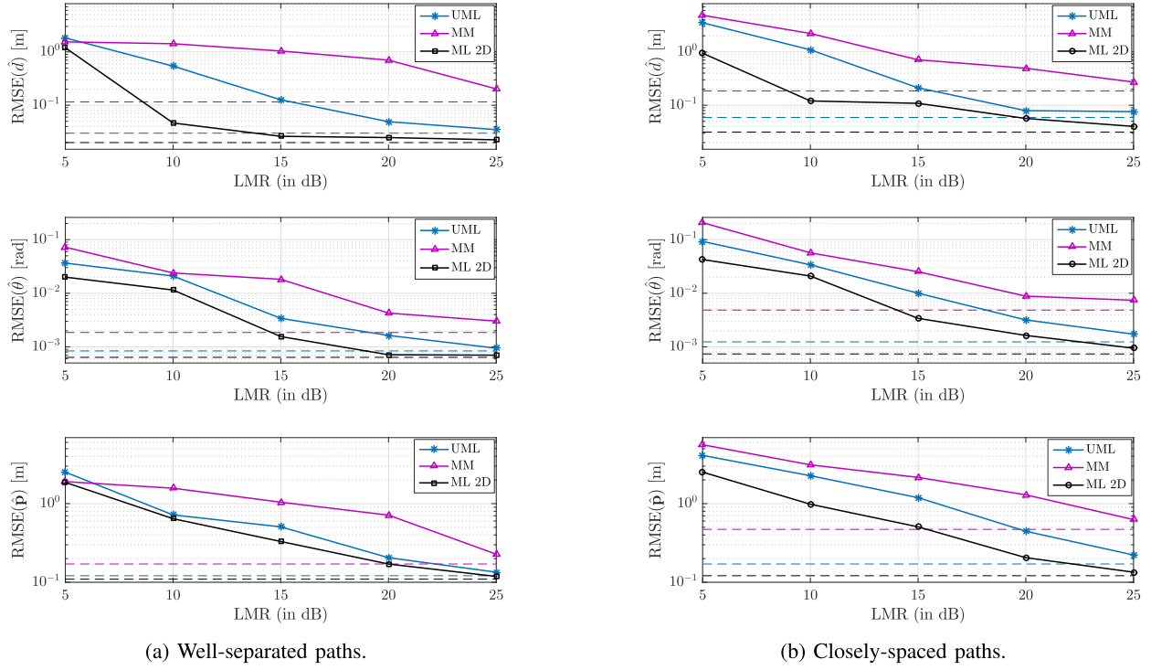
Fig. 6. RMSEs of the estimated d , \theta , and \mathbf{p} as function of the LMR for G = 10 and \text{SNR} = 15 dB for (a) well-separated and (b) closely-spaced paths. The dashed-curves represent LOS performance for reference.
